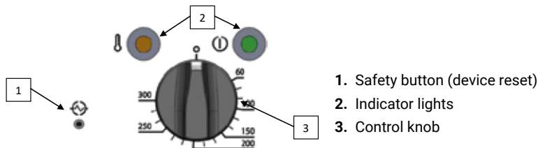
Figure 16. Device controls
