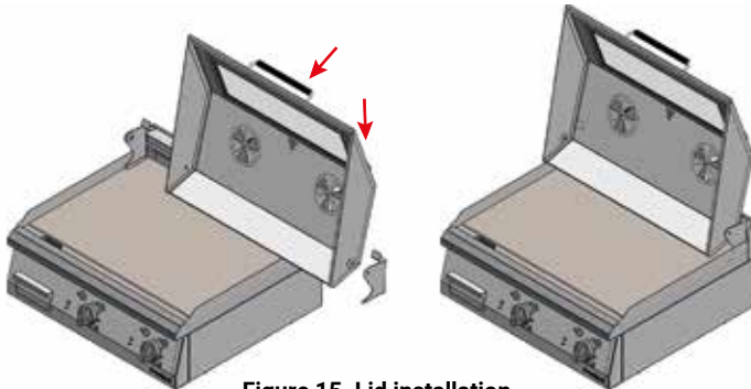
Figure 15. Lid installation.
