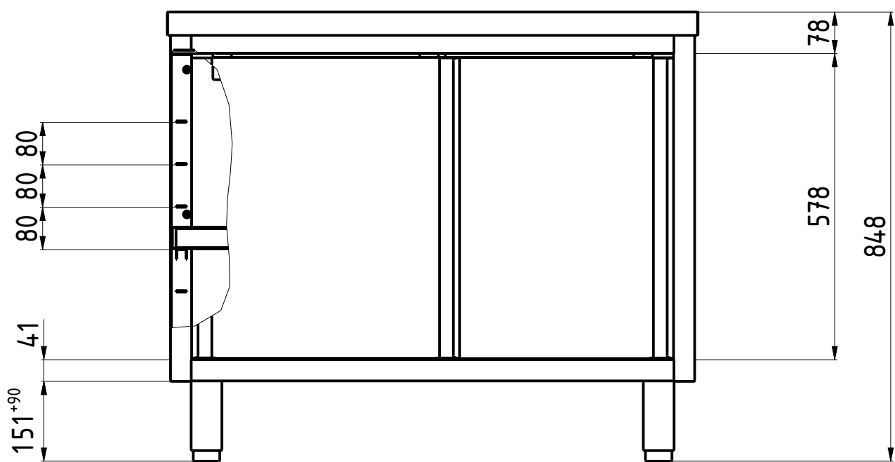
FRONT VIEW B-B 1:10
