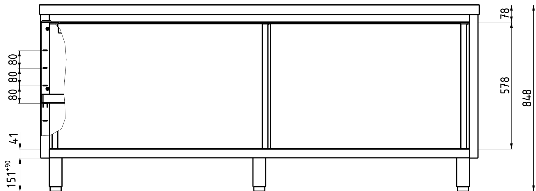
FRONT VIEW B-B 1:10
