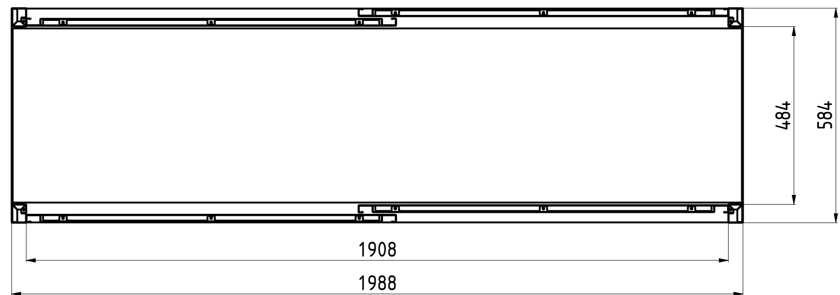
INTERNAL DIM C-C
