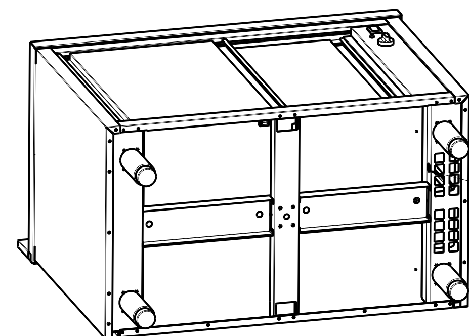
3D BOTTOM VIEW 1:10
